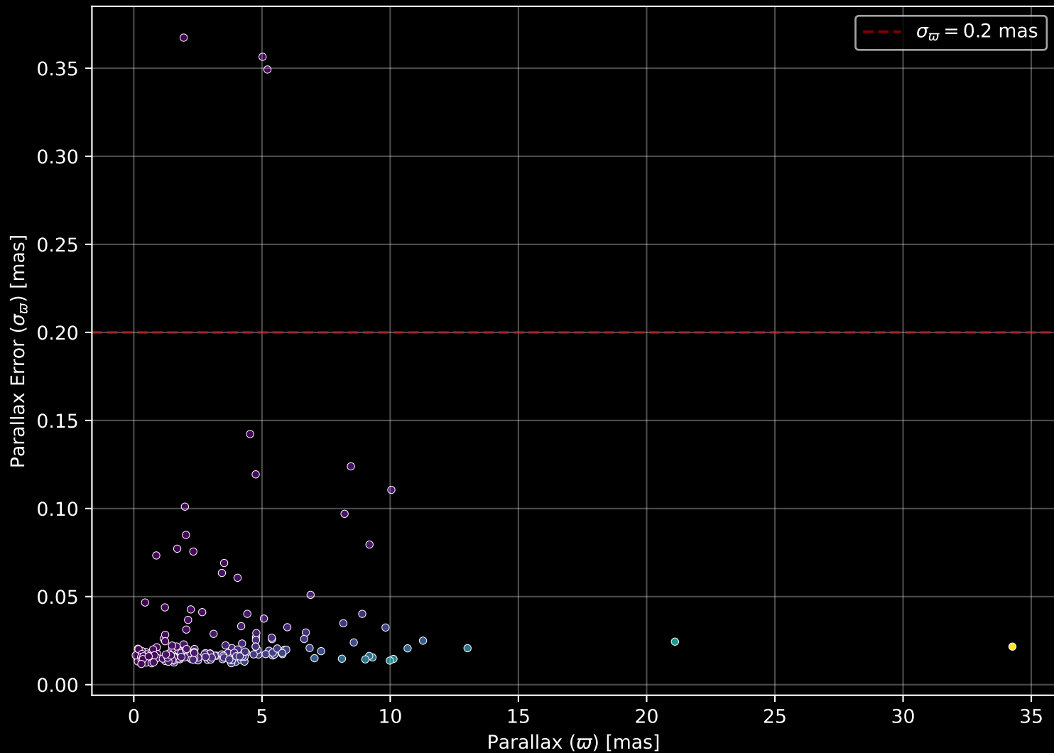
APOGEE DR17 Field: [356+50_MGA] Parallax Quality (n= 195)
