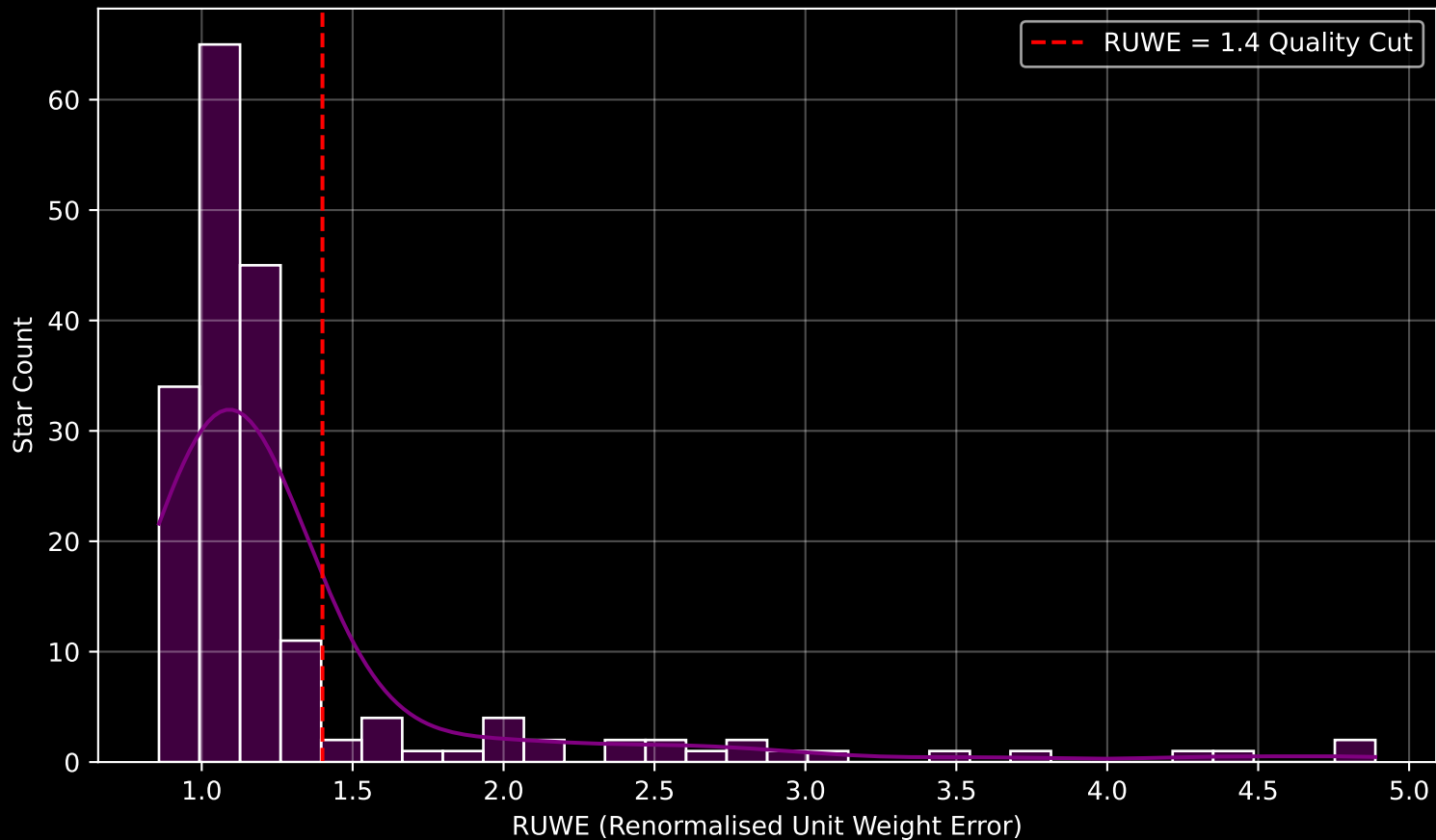
GAPOGEE DR17 Field [356+50_MGA] RUWE Distribution (n= 184)
