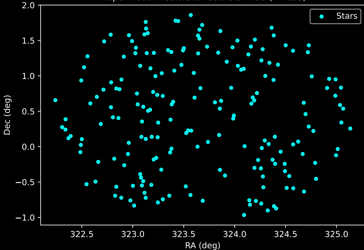
APOGEE DR17 Field: [356+50_MGA] Proper Motion Vectors for Gaia Star Field (n= 195)
