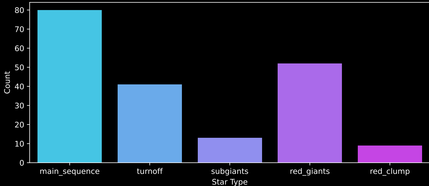
APOGEE DR17 Field: [356+50_MGA] Count plot of Star Type
