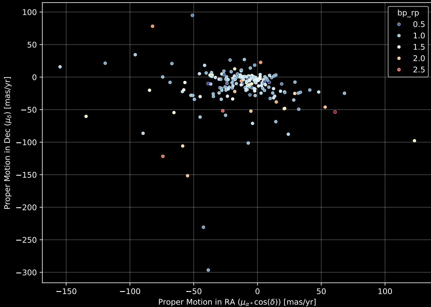
APOGEE DR17 Field: [356+50_MGA] Proper Motion Diagram (n= 195)
