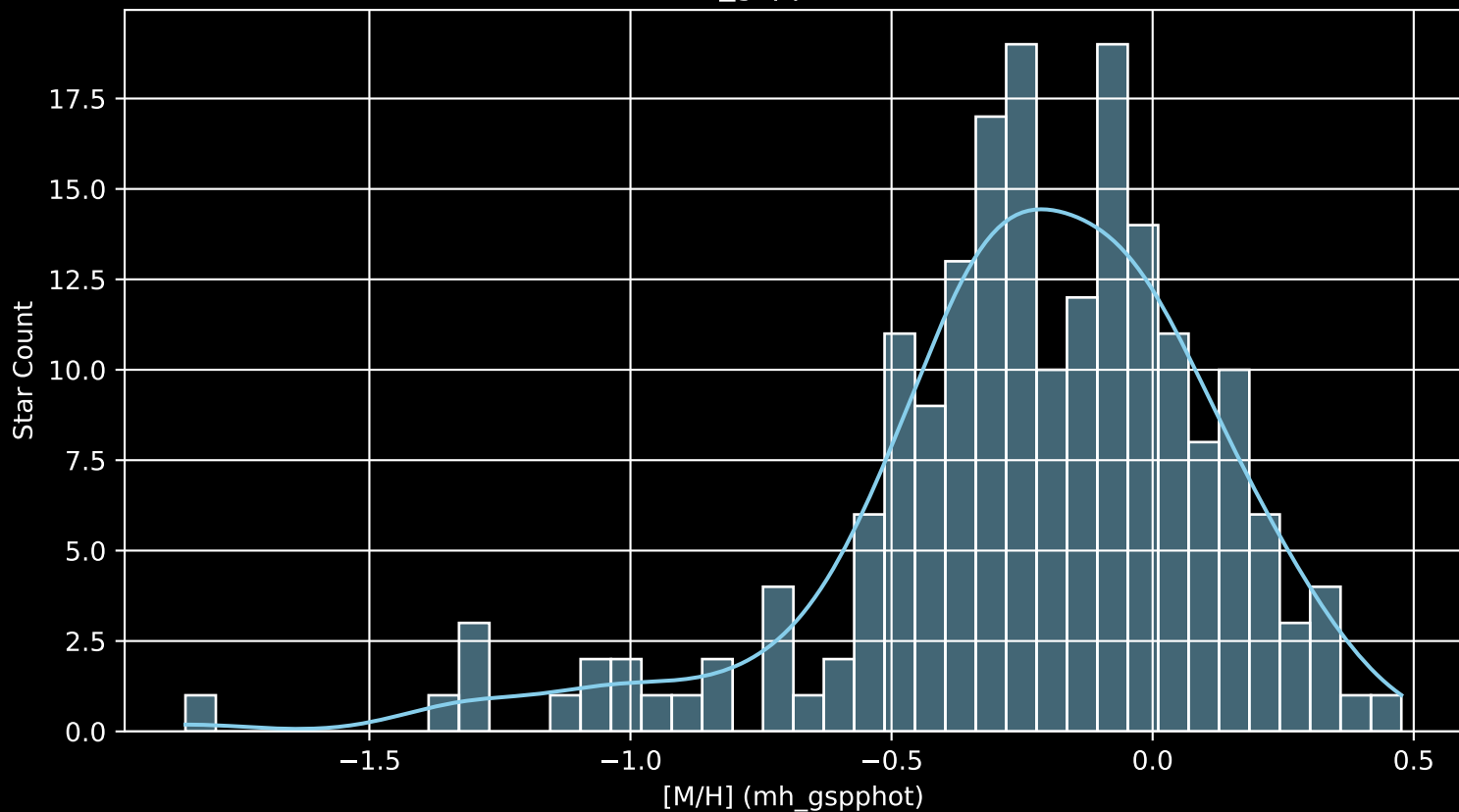
APOGEE DR17 Field: [356+50_MGA [M/H] (mh_gspphot) (n= 195)
